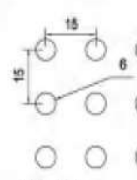
NA-009 ø 6 straight row spacing 15x15 Opening rate of 12.5% Available thickness 1.5-2.0
