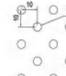
NA-027 ø 5 straight row spacing 20x10 Opening rate of 9.8% Available thickness 1.5-2.5
