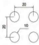
NA-001 ø 10 straight row spacing 20x20 Opening rate of 19.6% Available thickness 1.5-2.0
