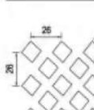
NA-043 Ling-shaped hole 15x15 26x26 straight row spacing Opening rate of 49% Available thickness 0.8-2.0
