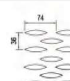
NA-039 53x11 olive-shaped hole Full hole spacing 74x18 Opening rate of 30% Available thickness 0.8-2.0
