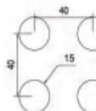
NA-004 ø 20 straight row spacing 40x40 Opening rate of 19.6% Available thickness 1.5-2.5
