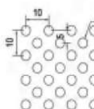
NA-022 ø 4 straight row spacing 10x5 Opening rate of 25.1% Available thickness 0.8-2.0
