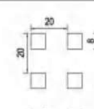
NA-046 8x8 square hole Straight row spacing 20x20 Opening rate of 19% Available thickness 1.5-2.0
