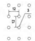
NA-018 ø 3 straight row spacing 12x12 Opening rate of 4.9% Available thickness 0.8-2.0
