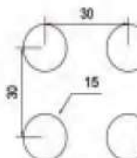
NA-003 ø 15 straight row spacing 30x30 Opening rate of 19.6% Available thickness 1.0-2.5
