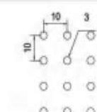
NA-034 ø 3 straight row spacing 10x10 Opening rate of 7% Available thickness 0.8-2.0
