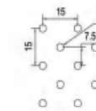
NA-019 ø 3 straight row spacing 15x7.5 Opening rate of 6% Available thickness 0.8-1.5
