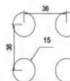
NA-006 ø 25 straight row spacing 36x36 Opening rate of 37.8% Available thickness 1.5-3.0
