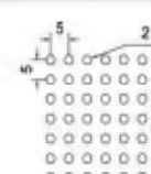
NA-031 ø 2.3 straight row spacing 5x5 Opening rate of 16.6% Available thickness 0.8-1.2
