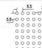
NA-033 ø 2.3 straight row spacing 5.5x5.5 Opening rate of 16.2% Available thickness 0.8-1.2
