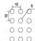
NA-023 ø 5 straight row spacing 10x10 Opening rate of 19.6% Available thickness 0.8-3.0
