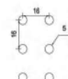
NA-025 ø 5 straight row spacing 16x16 Opening rate of 7.8% Available thickness 1.5-3.0
