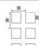
NA-045 20x20 30x30 square hole Straight row spacing Opening rate of 44% Available thickness 1.5-3.0
