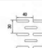
NA-037 30x5 rounded hole Full hole spacing 40x15 Opening rate of 22% Available thickness 0.8-2.0
