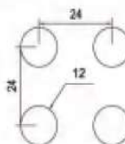
NA-002 ø 12 straight row spacing 24x24 Opening rate of 19.6% Available thickness 1.5-2.0
