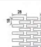
NA-042 21x4 28x9 rectangular hole straight row spacing Opening rate of 16% Available thickness 0.8-1.5
