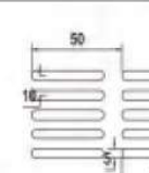
NA-048 40x5 rounded vertical hole spacing 50x10 Opening rate of 8% Available thickness 1.5-3.0
