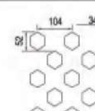
NA-047 Outer diameter of 34 hexagonal hole Full hole spacing 104x32 Opening rate of 19% Available thickness 1.5-3.0
