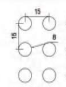
NA-013 ø 8 straight row spacing 15x15 Opening rate of 22.3% Available thickness 1.5-2.5
