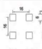
NA-036 6x6 vertical spacing of 16x16 square hole Opening rate of 14% Available thickness 0.8-2.0
