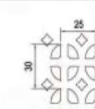
NA-040 20x24 flower-shaped hole straight row spacing 25x30 Opening rate of 25% Available thickness 1.5-3.0
