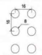
NA-014 ø 8 straight row spacing 16x16 Opening rate of 19.6% Available thickness 1.5-2.5
