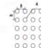
NA-020 ø 4 straight row spacing 8x8 Opening rate of 19.6% Available thickness 0.8-2.0
