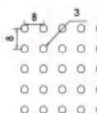
NA-015 ø 3 straight row spacing 6x6 Opening rate of 11% Available thickness 0.8-2.5
