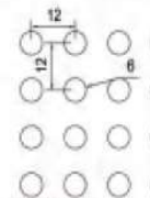
NA-008 ø 6 straight row spacing 12x12 Opening rate of 19.6% Available thickness 1.5-2.0
