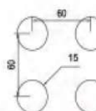
NA-005 ø 20 straight row spacing 60x60 Opening rate of 8.7% Available thickness 1.5-2.5
