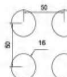
NA-007 ø 30 straight row spacing 50x50 Opening rate of 28.2% Available thickness 1.5-3.0
