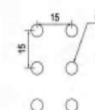
NA-024 ø 5 straight row spacing 15x15 Opening rate of 8.7% Available thickness 1.5-3.0
