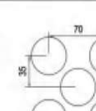
NA-049 ø 40 straight row spacing 70x35 Opening rate of 28.2% Available thickness 1.5-3.0
