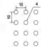
NA-021 ø 4 straight row spacing 10x10 Opening rate of 12.5% Available thickness 0.8-2.5
