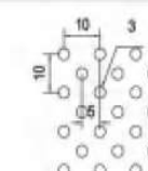
NA-035 ø 3 straight row spacing 10x5 Opening rate of 14% Available thickness 0.8-2.0
