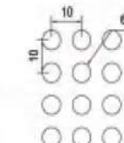
NA-028 ø 6 straight row spacing 10x10 Opening rate of 28.2% Available thickness 0.8-1.5
