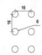
NA-010 ø 6 straight row spacing 16x16 Opening rate of 11% Available thickness 1.5-2.0
